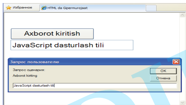
7.3-rasm. Prompt metodining qo'llanilishi natijasi 57 .
