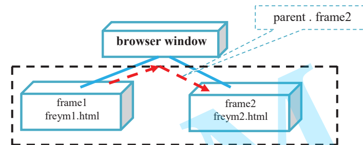
7.10-rasm. Quyi pog‘onada turgan 1-freymdan2-freymga murojaat 65 .
