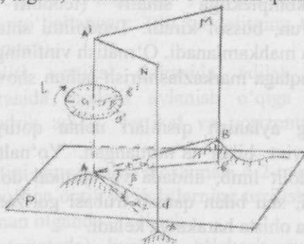
4.1-rasm. Gorizontal burchak o'lchash sxemasi
