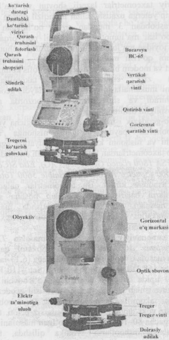
6.13-rasm. Elektron taxeometr
