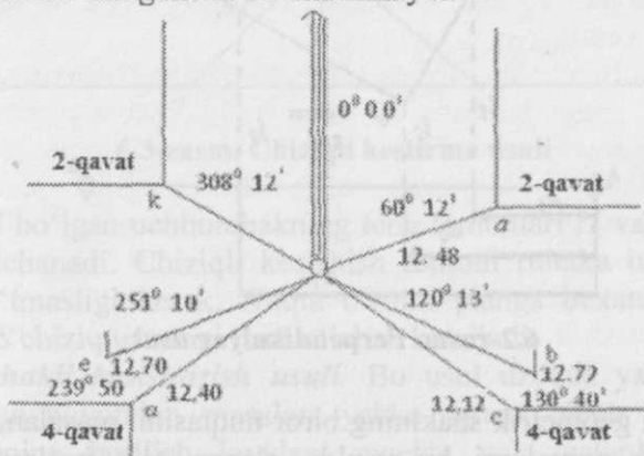
6.1-rasm. Qutbiy usulda planga olish
