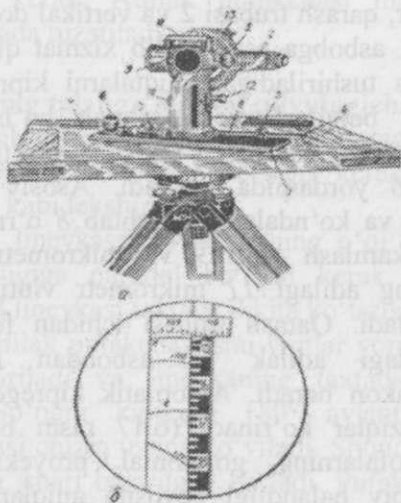
6.17-rasm. KA2-kipregeli
