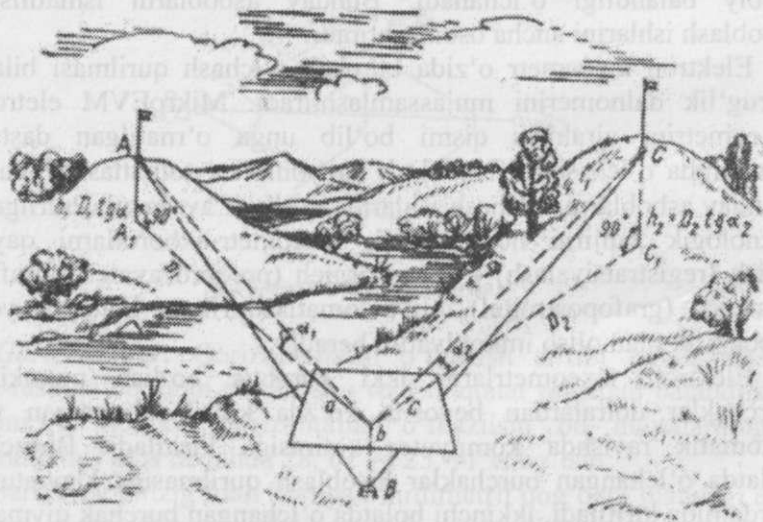
6.16-rasm. Grafik usulda plan olish
