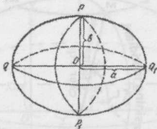
1.2-rasm. Ellipsoid
