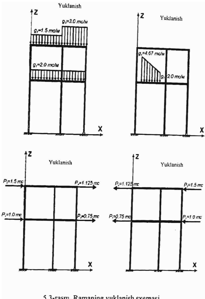
5.3-rasm. Ramaning yuklanish sxemasi.
