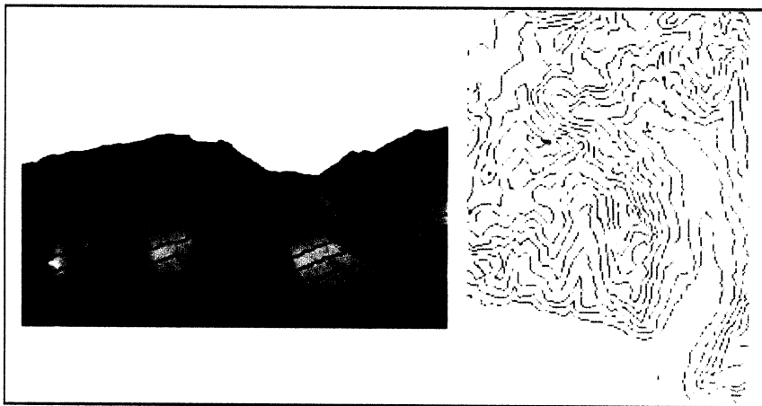
5.1-rasm. O'zgarmas balandlikka ega gorizontall yuza (chapda), gorizontallar kartasi (o'ngda)
