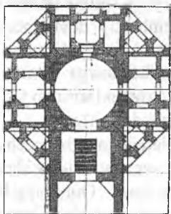
XVI asrda buxorolik noma'lum muhandis tomonidan chizilgan sardoba tarhi (loyihasi).
