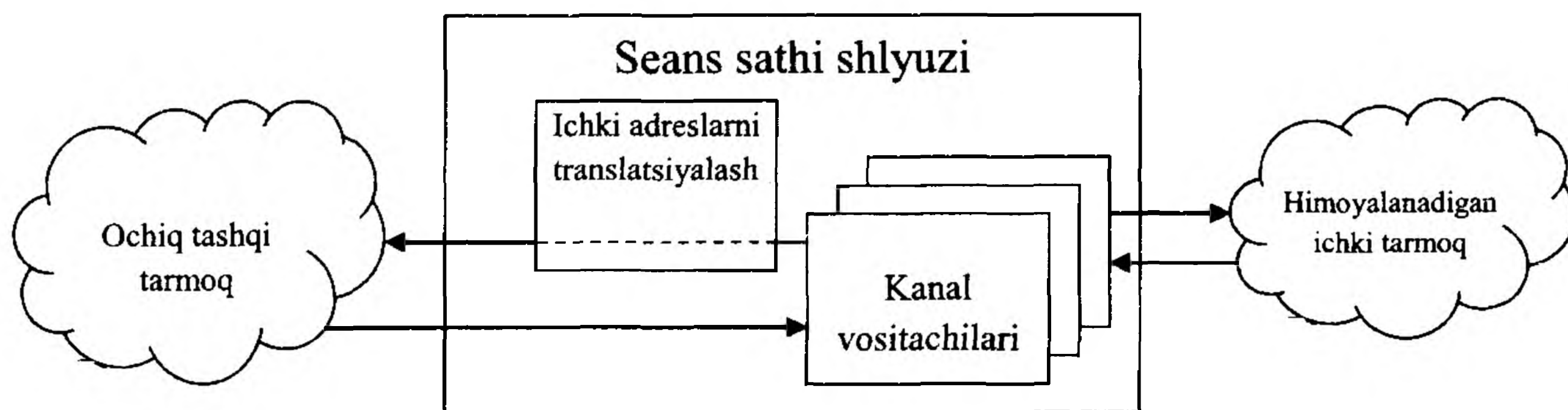
8.8-rasm. Seans sathi shlyuzining ishlash sxemasi.
