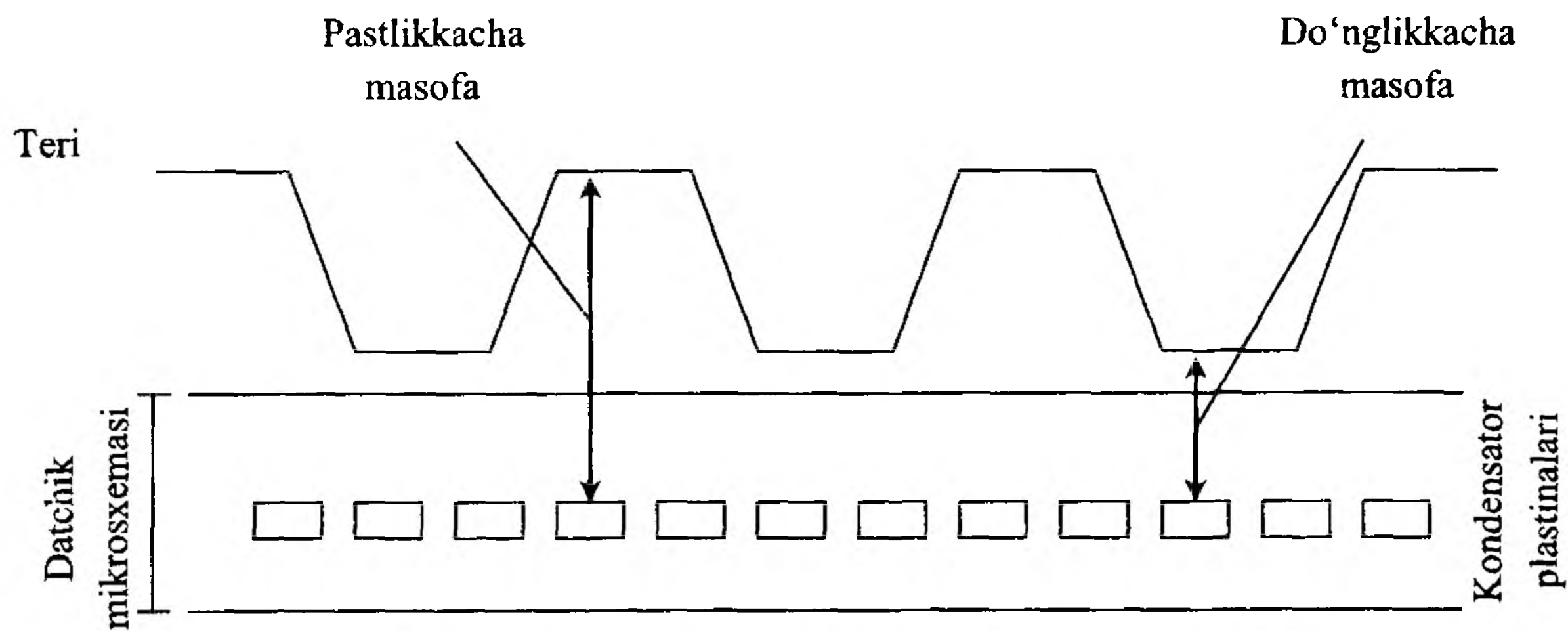
6.6-rasm. Sensor ishlashining prinsipi.
