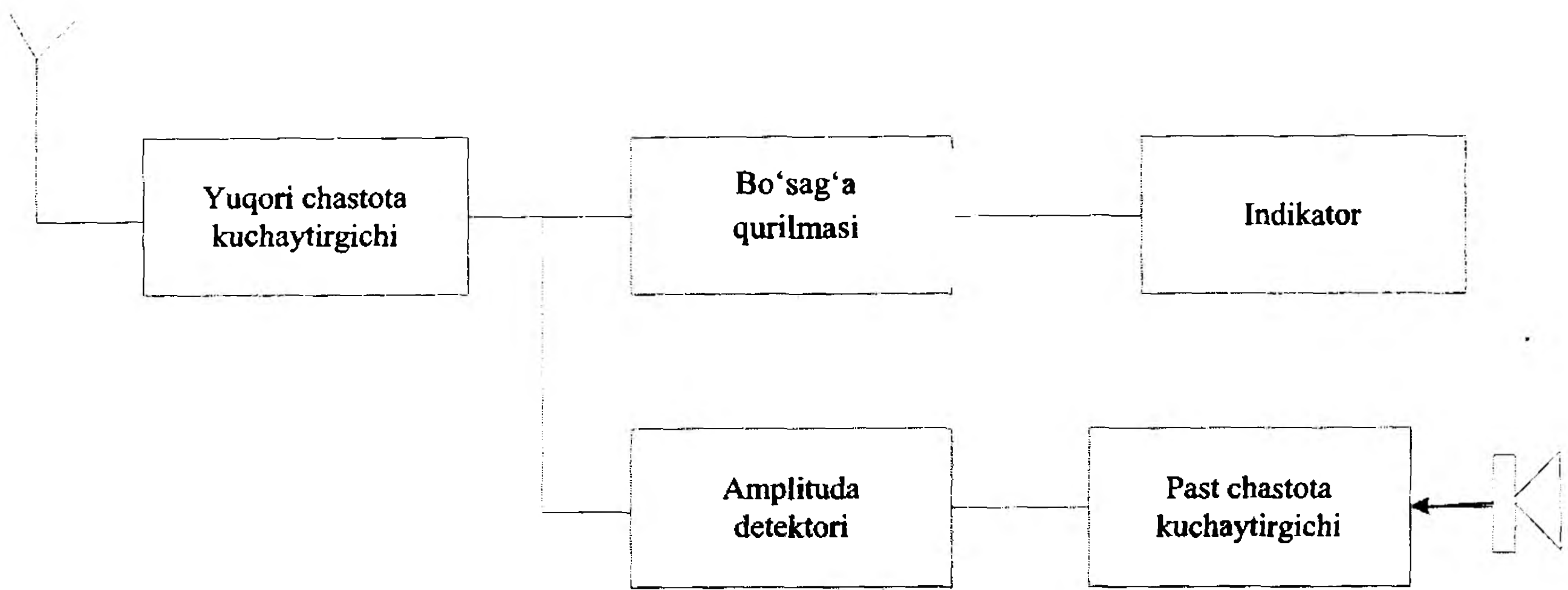
10.4-rasm. Elektromagnit nurlanish indikatorining sxemasi.
