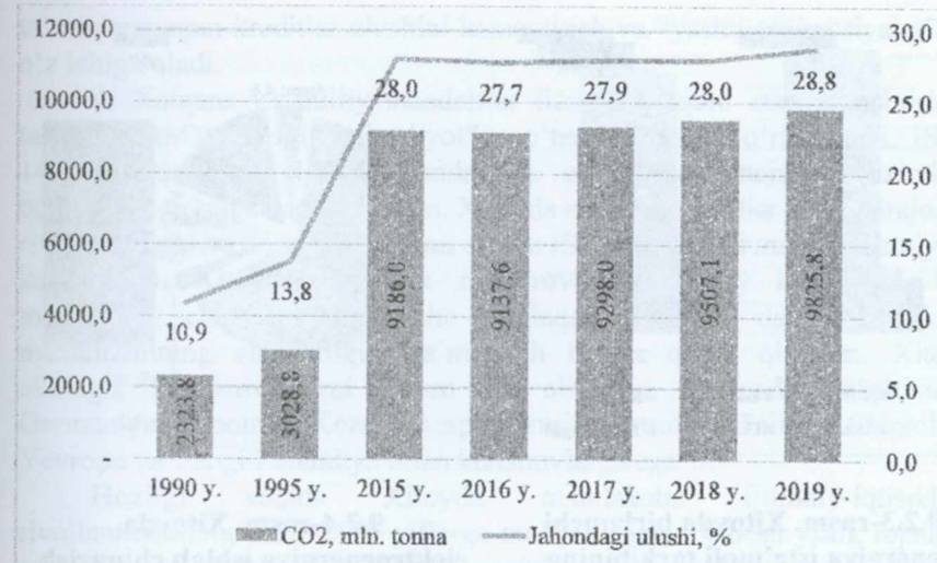
9.2.2-rasm. Xitoyda atmosferaga chiqarilayotgan CO 2 miqdoriging o'zgarishi 268
